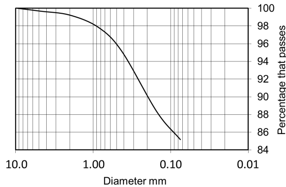
Figure 2. Granulometric curve of the material.
