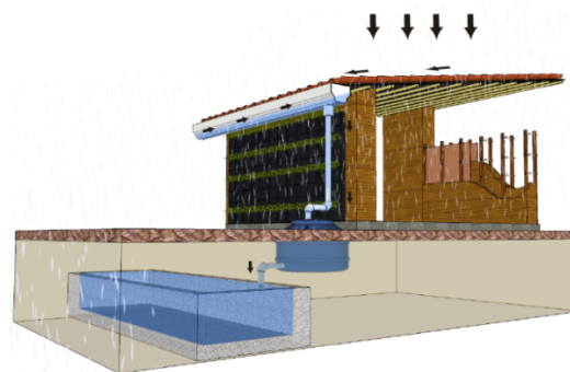
Figure 6. Diagram of the water collection and use process.
