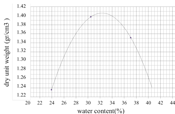
Figure 3. Compaction curve.
