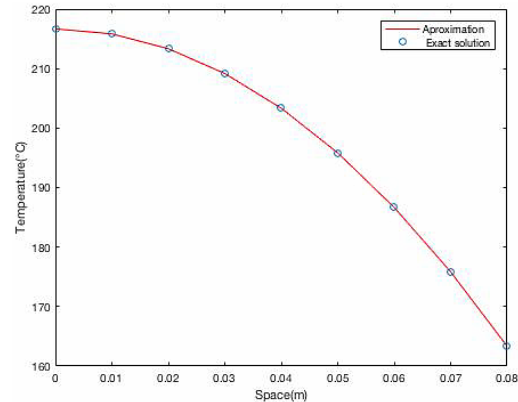
Figure 1. Contour of temperature with the method of linear algebra and exact solution.
