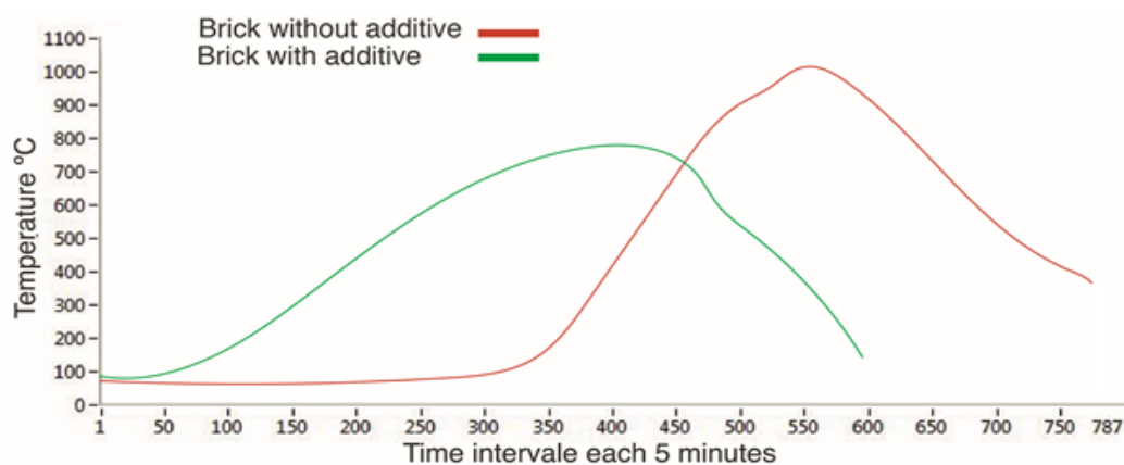
Figure 1. Temperature profile on the brick located in the central part of the kiln.
