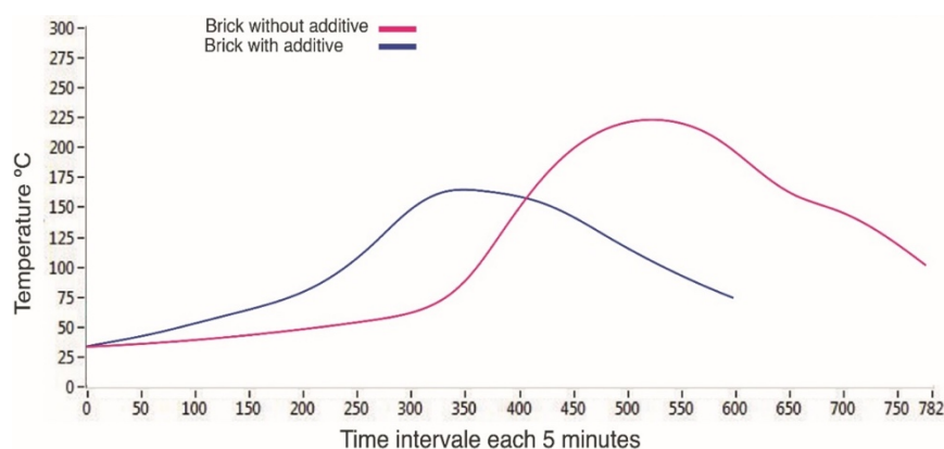
Figure 2. Temperature profile of gases emitted to the environment.
