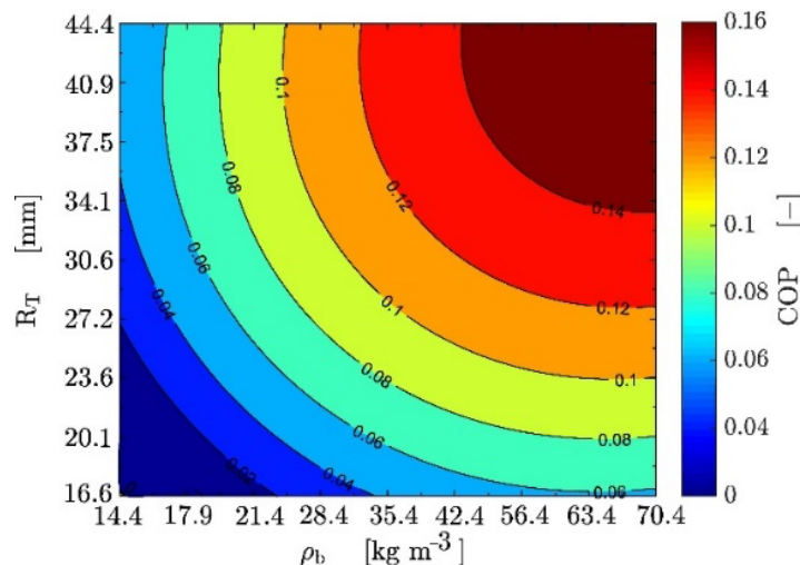
Figure 4. Variation of COP as a function of the radius of the reactor tube and the specific bulk density of the adsorbent bed for a cycle time of 30 minutes.
