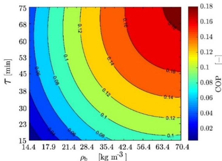
Figure 2. Variation of COP as a function of cycle time and specific bulk density of the adsorbent bed for a reactor tube radius of 30.6 mm.
