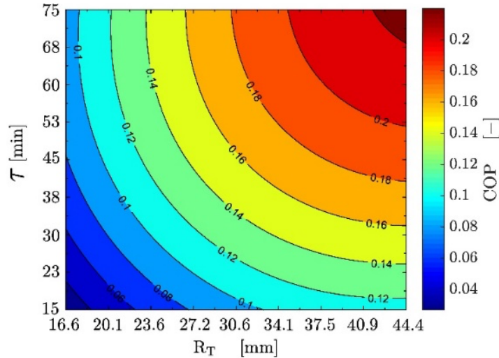
Figure 3. COP variation as a function of the cycle time and radius of the reactor tube for adsorbent apparent density of 59 \text{ kg m}^{-3} .
