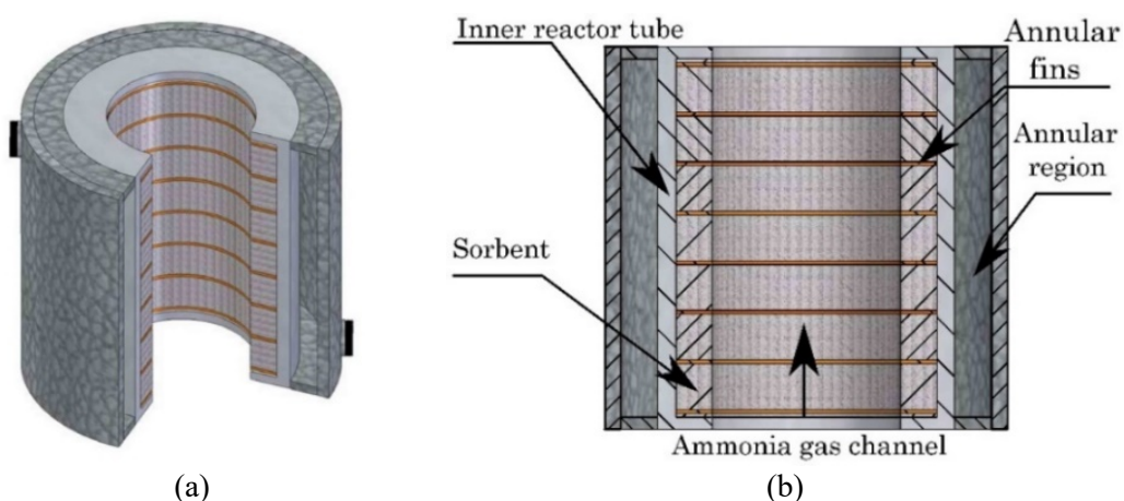
Figure 1. Reactor of the chemical adsorption refrigeration system (a) Isometric view of the reactor and (b) Reactor components.
