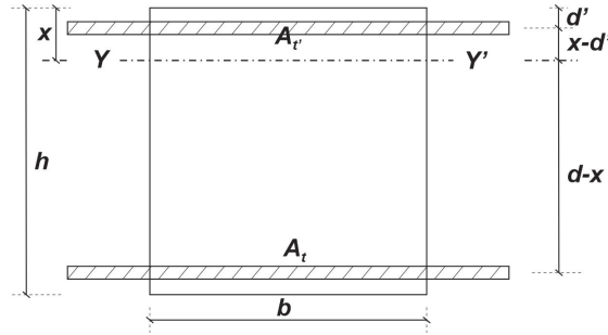
Figure 8. Transformed cross-section of a doubly reinforced rectangular beam.
