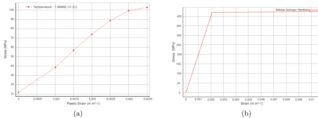
Figure 4. Behavior of concrete and steel, (a) multilinear hardening model of concrete, and (b) bilinear model of reinforcing steel.
