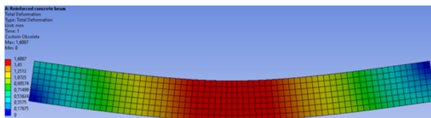
Figure 7. Displacement in the Z-direction.
