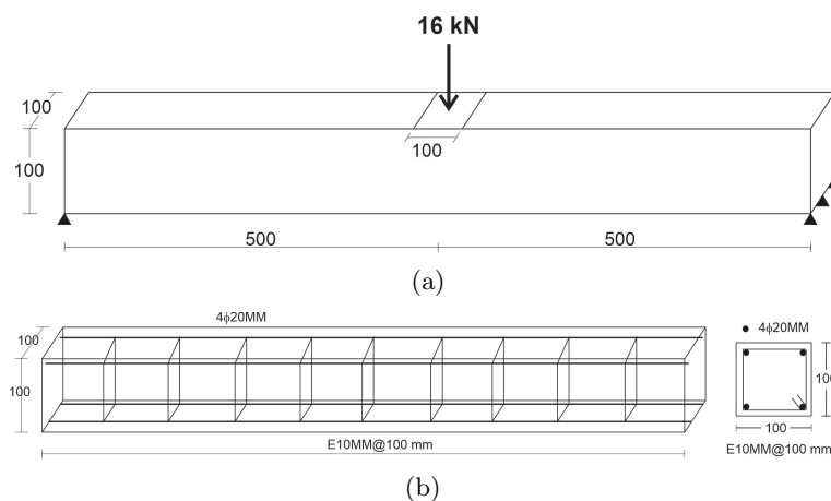
Figure 1. Model of reinforced concrete beam, (a) loading and boundary conditions and (b) schematic representation of the longitudinal and transverse reinforcement of the beam.
