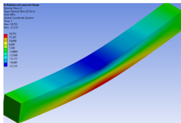
Figure 6. Normal stresses in the z-direction.
