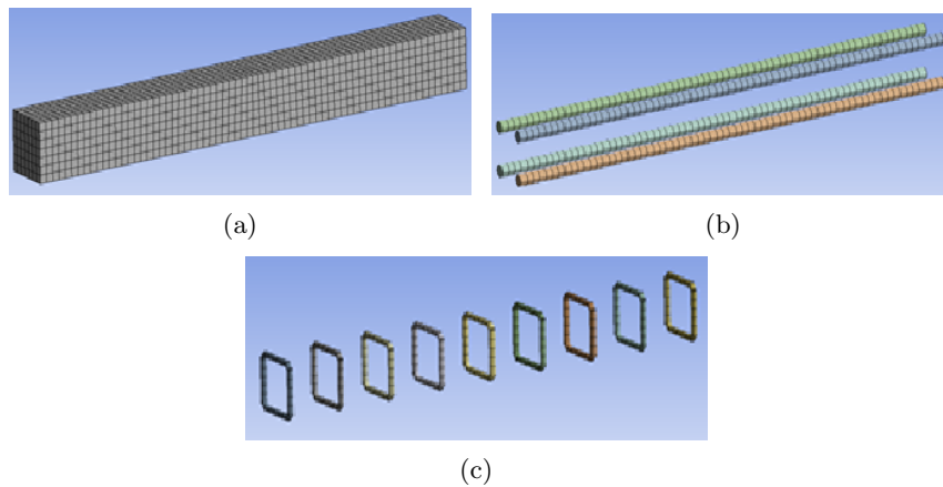
Figure 5. Discretization of the model, (a) concrete beam, (b) longitudinal reinforcement and (c) transverse reinforcement.
