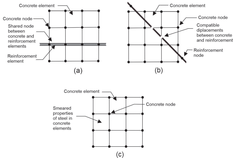
Figure 2. Models for reinforcement of reinforced concrete materials: (a) discrete model, (b) embedded model, and (c) smeared model. Adapted from [10].
